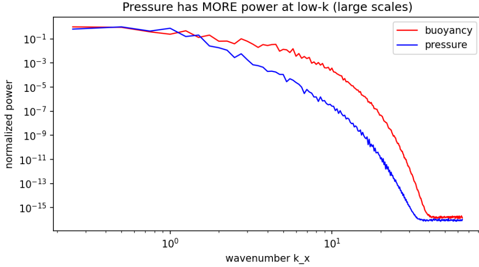
Figure 5. Spatial spectra: shared energy-containing scale; \sim 10^4 \times high- k gap — the 1/k^4 elliptic suppression.
