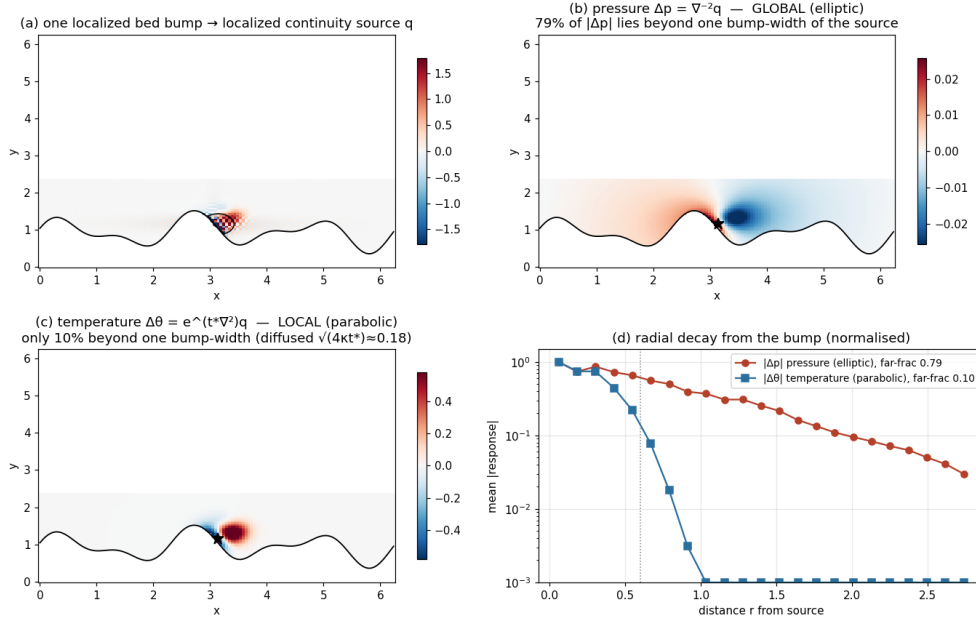
Figure 6. Identical localized source, two operators: global \ln r elliptic response (79% beyond one bump-width) vs confined Gaussian parabolic response.
