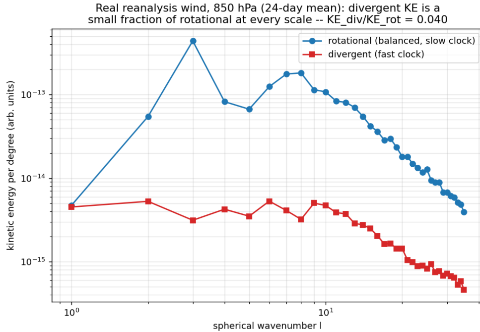
Figure 13. Kinetic-energy spectra by spherical wavenumber: the divergent branch 1–2 decades below the
