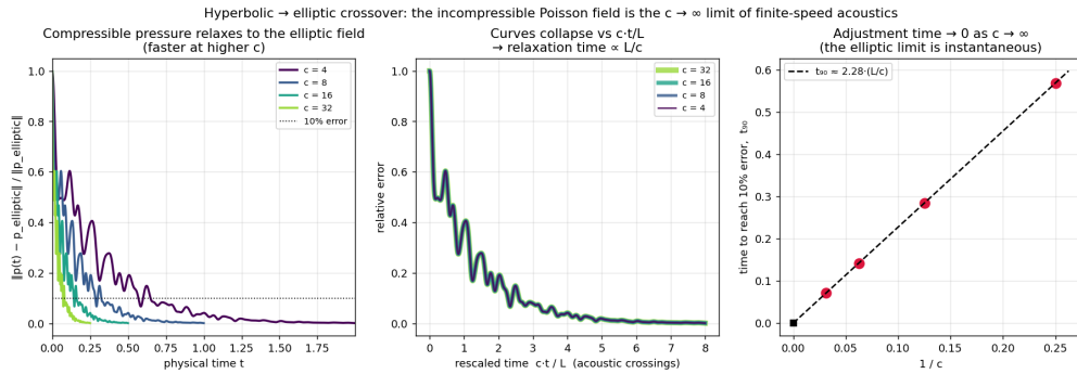
Figure 7. Crossover: relaxation of the compressible pressure to the elliptic field; all c collapse in ct/L ; t_{90} \approx 2.3 L/c .
